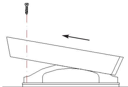
1. Rear screws / Hintere Schrauben
